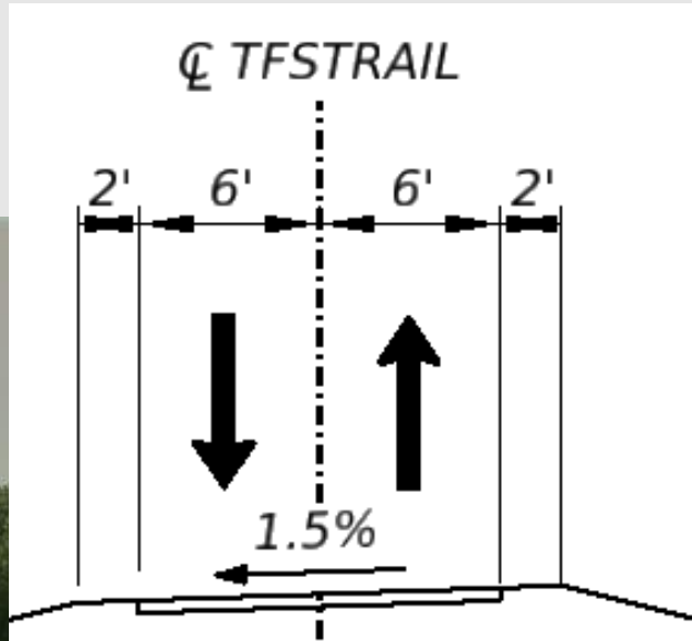
At grade section
