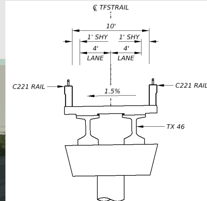
Bridge Section
