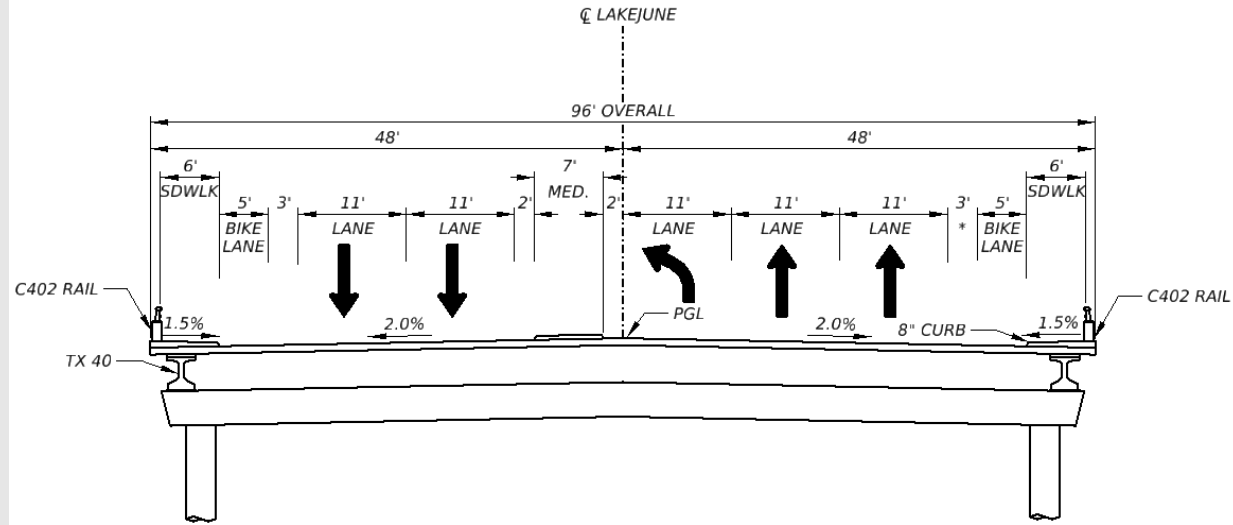
LAKE JUNE RD COMPLETED TYPICAL SECTION
