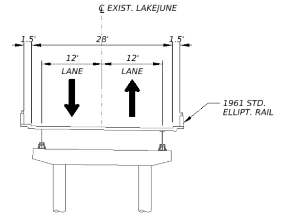
LAKE JUNE RD EXISTING TYPICAL SECTION EXISTING BRIDGE TO BE REMOVED
