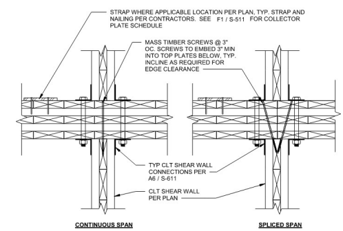
Typ. CLT Floor
