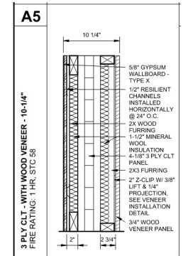
Interior Wall Detail
